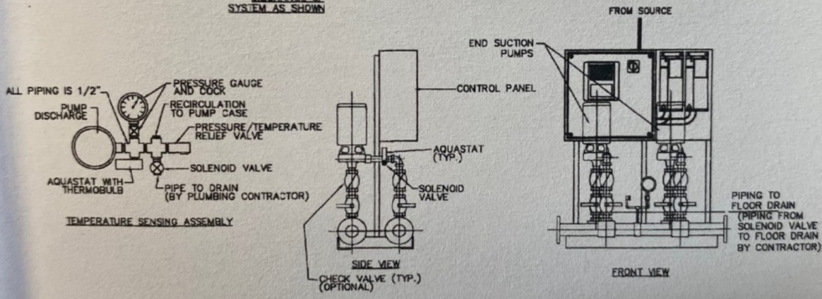
BOOSTER PUMP DETAIL NOT TO SCALE
